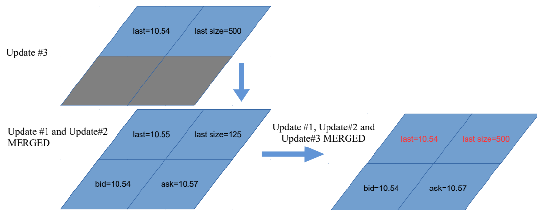
Figure 6– All the three updates are merged together.
